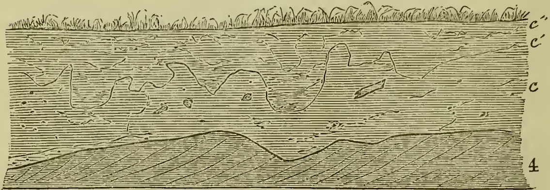
Fig. 7.—Section at the Brick-earth pit, Limpsfield Common.
